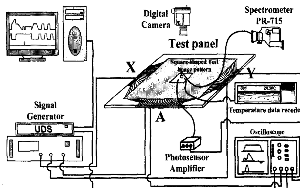
Fig. 1. Schematic diagram of experimental setup employed in this research.
