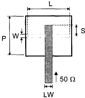
Fig. 3 Configuration of single antenna element.
