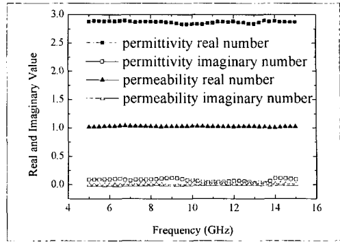
Fig. 2 Permittivity and permeability of adhesive film.
