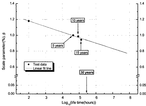
Fig. 11 Log scale plot of Weibull scale parameter and aging time for fiber failure strain.
