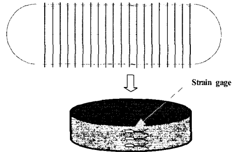
Fig. 4 Hoop ring specimen from composite pressure vessel.
