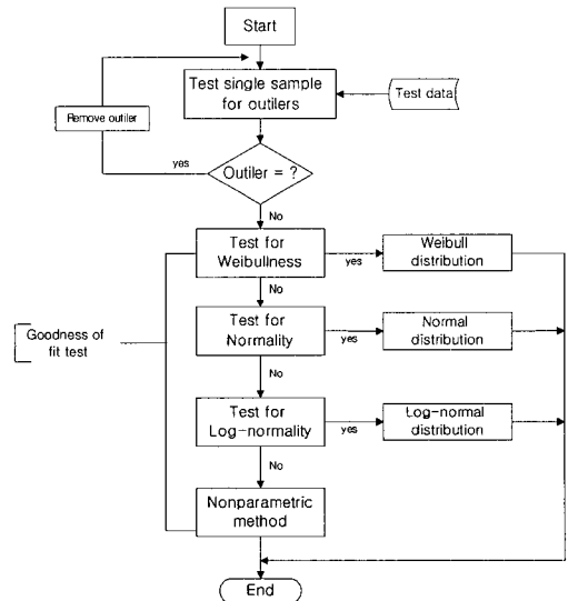
Fig. 9 Flowchart illustrating procedure for goodness of fit test.
