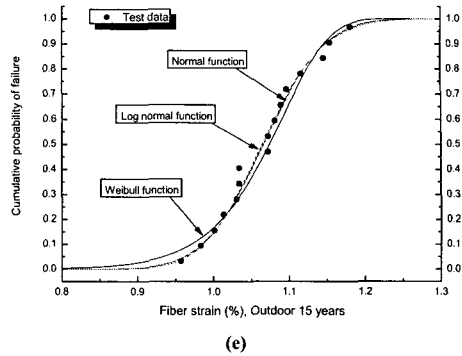
Fig. 10 Comparison of predicted cumulative distribution function and test data: (a) baseline specimens; (b) 10 year aged specimens (indoor); (c) 15 year aged specimens (indoor); (d) 10 year aged specimens (out-door); (e) 15 year aged specimens (out-door).
