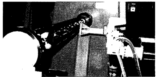
Fig. 2 Filament winding using the 4-axis winding machine.
