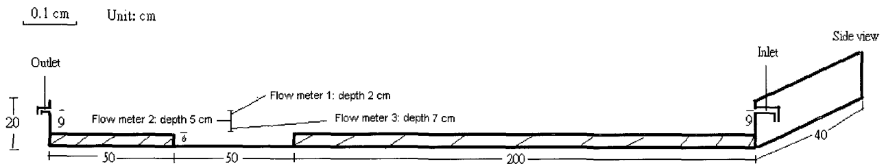
Fig. 1. The setup of the flume apparatus. Note that the depth of the flow meter position is denoted from the water surface.
