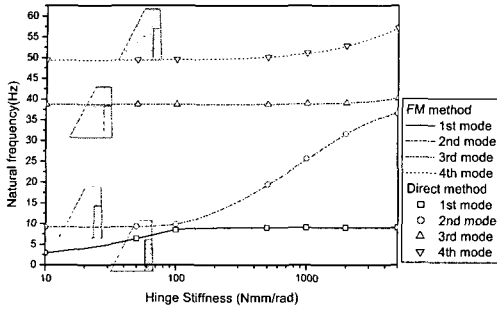
Fig. 3 Variation of natural frequency of Aluminum wing with control surface as hinge stiffness increases.
