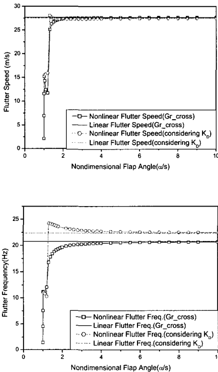
Fig. 11 Nonlinear flutter characteristics of composite wing with control surface considering dynamic stiffness([02/90]₂s).
