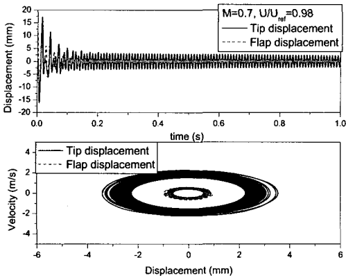
Fig. 8 Time history and phase plot of wing with control surface.
