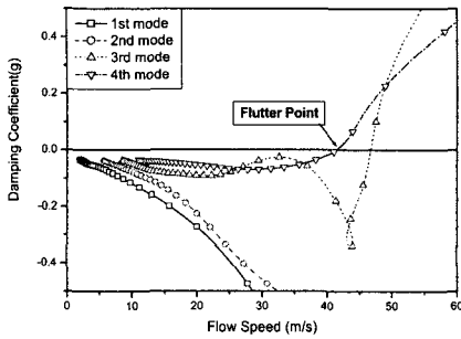
Fig. 6 V-g plot of aluminum wing with control surface.
