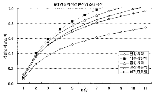
Fig. 4. Depletion curve ratio of SCA using non linear regression by five river basins in South Korea.
