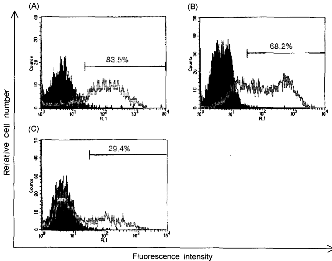
Fig. 4. Representative flow cytometric histograms illustrating the expression of Gb3 in Vero cells (A), DC2.4 cells (B) and Raw264.7 cells (C). Cells were incubated for 24 hrs at 37°C in the culture medium containing 0.5% FBS. After incubation, the SLT-I B-FITC labeled cells. Data is representative of two experiments.
