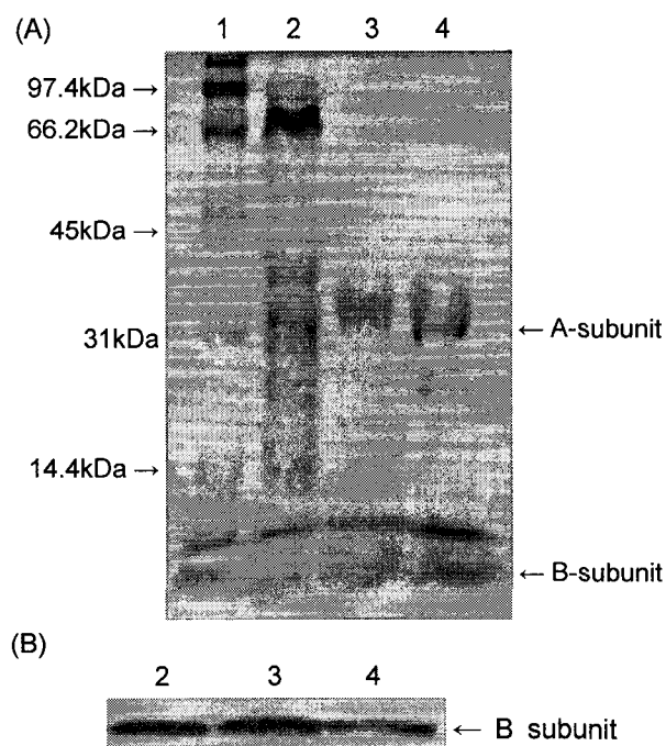
Fig. 1. (A) SDS-PAGE analysis of SLT-I from E. coli O157 (ATCC 43890). The samples were analyzed on 15% polyacrylamide gels. The arrows on the right hand side of the figure indicate the location of the A and B subunit bands. (B) An immunoblotting assay of purified SLT-I was conducted using anti-B mAb as the secondary antibody. The positions of the standard proteins used to calibrate the gels are indicated by their molecular weights on the left hand side of the Fig. 1, molecular size marker; 2, ammonium sulfate precipitated proteins; 3, Matrix gel green A pool of fractions; 4, purified SLT-I.
