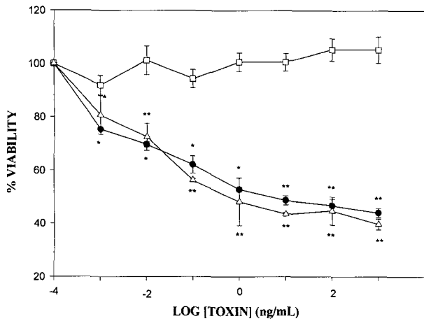
Fig. 3. Comparative cytotoxicities of SLT-I for Raw264.7 cells, DC2.4 cells and Vero cells. Cells were incubated with 10-fold dilutions of the toxins in 96-wells for 48 hrs at 37°C in humidified 5% CO 2 . Viability was measured by the uptake of MTT. Untreated cells were used to determine percent viability (□, Raw264.7 cells; ●, DC2.4 cells; △, Vero cells). The data shown is the averages of two separate experiments. Statistical significance: * p < 0.05 and ** p < 0.01 vs. non-treatment values. Values are mean ± S.D., n=6.
