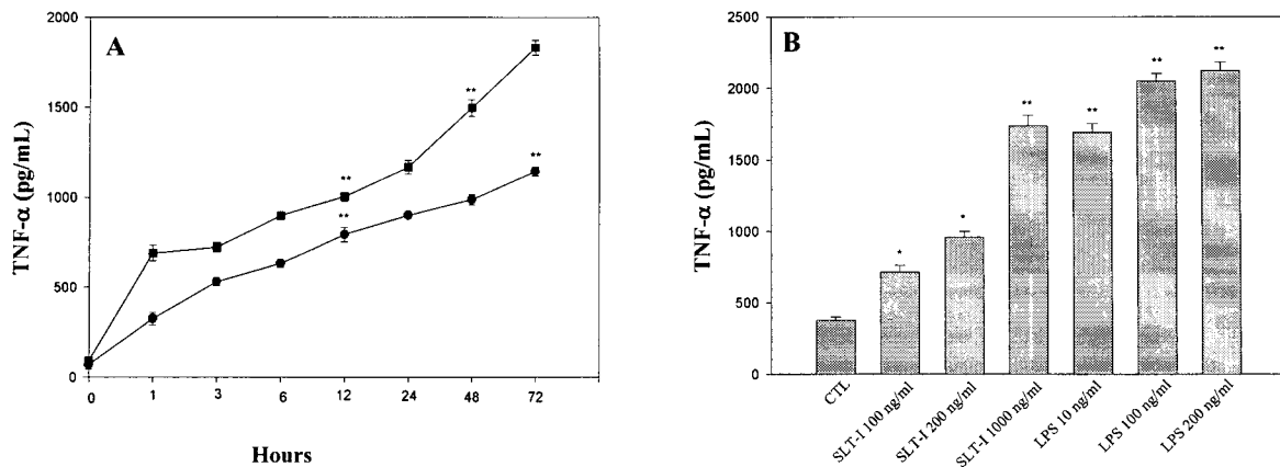
Fig. 5. Time- (A) and dose-dependent (B) TNF- \alpha production by Raw264.7 cells stimulated by SLT-I and LPS. Raw264.7 cells were stimulated by 200 \mu g/ml of SLT-I (■) and 100 ng/ml of LPS (●) for 72 hrs at 37°C in a humidified 5% CO 2 incubator (A). To evaluate dose- dependent TNF- \alpha production, Raw264.7 cells were stimulated by SLT-I (100, 200, and 1000 ng/ml) or LPS (10, 100, and 200 ng/ml) for 24 hrs. TNF- \alpha activities in the culture supernatants from Raw264.7 cells were measured as described in Materials and Methods. Significance was determined using the Student t -test versus the control group (* p < 0.05 and ** p < 0.01).
