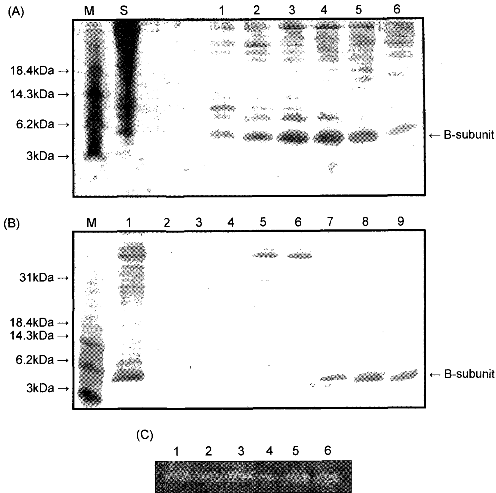
Fig. 2. (A) Anion exchange chromatography SLT-I B from 12-liters of culture supernatant of E. coli JM105 on Q-Sepharose column (1.6 x 30 cm). The column was eluted with 50 mM of Tris-HCl (pH 7.4). An SDS-PAGE analysis of anion exchange-purified SLT I B was conducted. M: molecular weight marker; s: crude sample; 1: fraction no. 28; 2: fraction no. 29; 3: fraction no. 30; 4: fraction no. 31; 5: fraction no. 32; 6: fraction no. 33. (B) Gel filtration (a) of SLT-I B from 12-liters of culture supernatant of E. coli JM105 on Sephacryl S-200 column (1.5 x 100 cm). The column was eluted with 10 mM of NaCl containing 50 mM of Tris-HCl (pH 7.4). An SDS-PAGE analysis of gel filtration-purified SLT I B was conducted. The samples were analyzed on 15% polyacrylamide gels. The arrows on the right-hand side of the figure indicate the location of the SLT-I B bands. The positions of the standard proteins used to calibrate the gels are indicated by their molecular weights on the left hand side of the figure. M: molecular weight marker; s: crude sample; 1: fraction no. 28; 2: fraction no. 29; 3: fraction no. 30; 4: fraction no. 31; 5: fraction no. 32; 6: fraction no. 33; 7: fraction no. 28; 8: fraction no. 34; 9: fraction no. 35. (C) SLT-I-B was represented by immunoblotting assay after gel filtration and ion exchange chromatography. 1: fraction no. 29; 2: fraction no. 30; 3: fraction no. 31 after gel filtration chromatography; 7: fraction no. 28; 8: fraction no. 34; 9: fraction no. 35 after ion-exchange chromatography.
