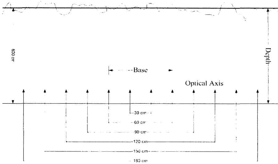
Fig. 5. Stereophotographing conditions with various base-depth ratios
