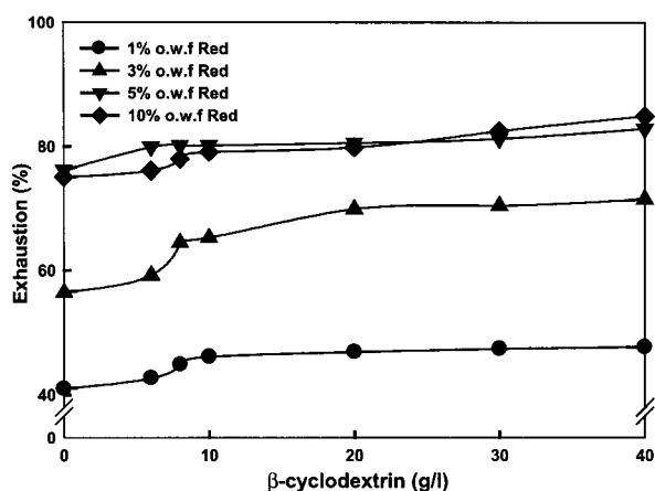
Fig. 5. Effect of \beta -cyclodextrin concentration on the %exhaustion of Berberine inclusion.
