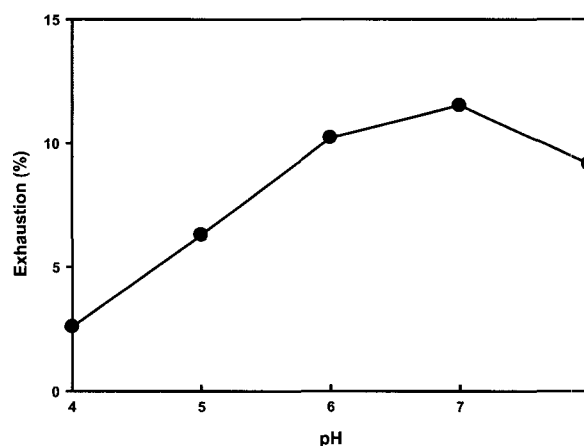
Fig. 4. Effect of pH on the %exhaustion of Berberine inclusion.
