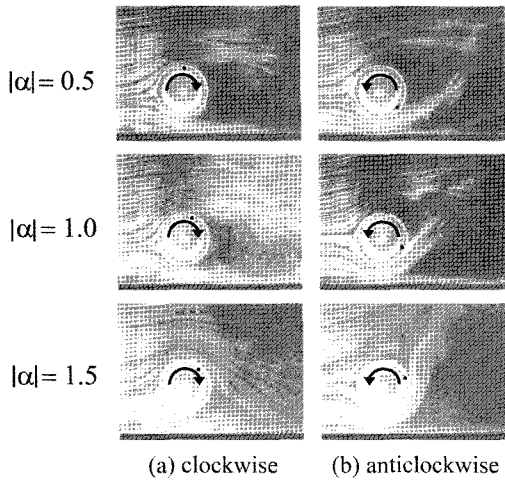
Fig. 10 Flow pattern around the rotating cylinder with velocity ratios ( H/D=0.4 , Re=0.7 \times 10^4 )
