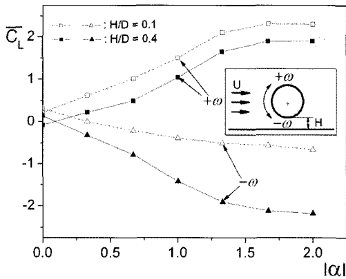
Fig. 8 Average lift coefficients of the rotating cylinder with velocity ratios ( Re=1.9 \times 10^4 )
