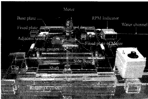
Fig. 3 Photo of driving system
