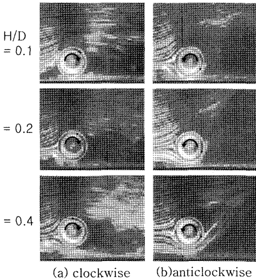
Fig. 7 Flow pattern around the rotating cylinder with H/D ( |\alpha|=1, Re=0.7 \times 10^4 )
