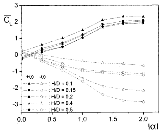
Fig. 9 Average lift coefficients of the rotating cylinder with H/D ( Re=1.9 \times 10^4 )
