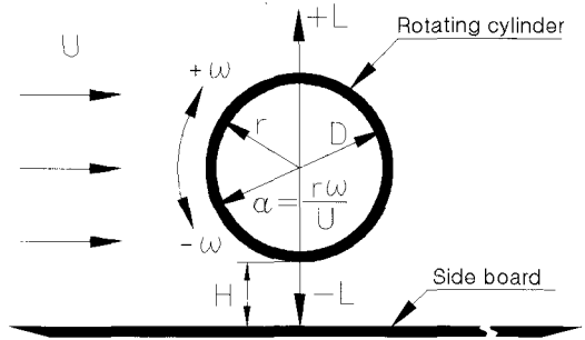
Fig. 1 Experimental model
