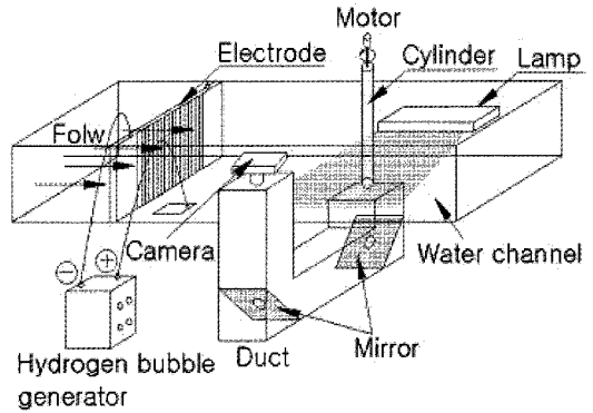
Fig. 4 Schematic structure of experimental apparatus for flow visualization
