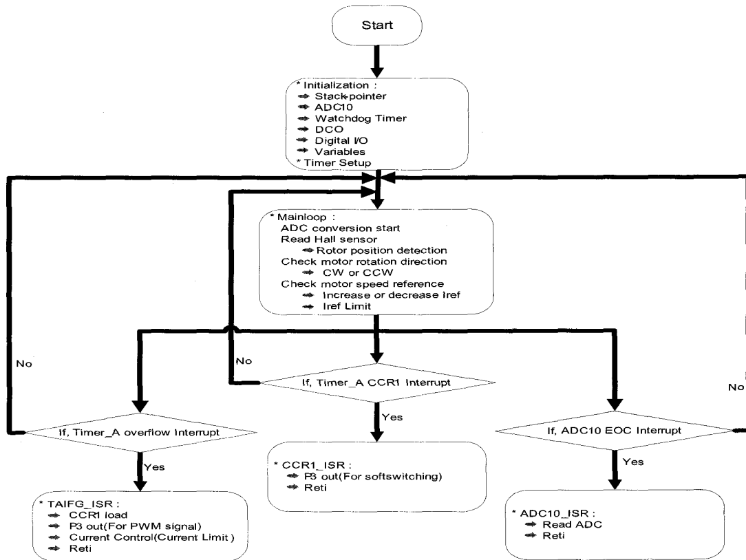
Fig. 5 Software flowchart.
