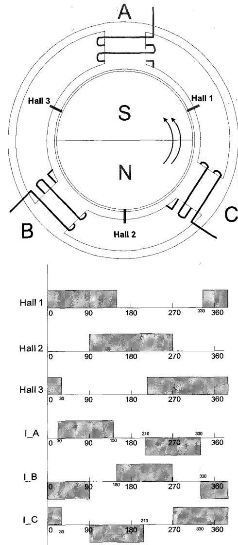
Fig. 2 BLDC motor structure and signals
