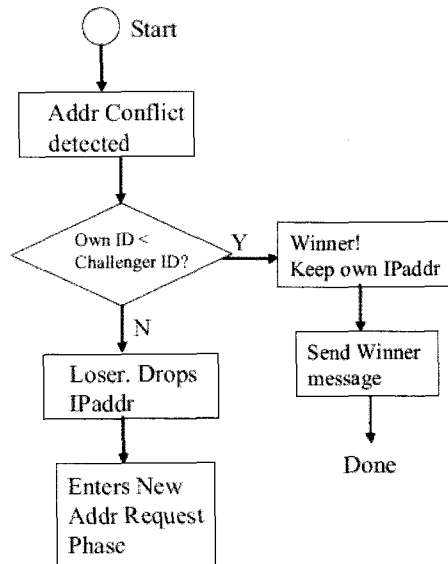
(b) LiA 주소 충돌 해결 (b) LiA Address Collision Resolution
