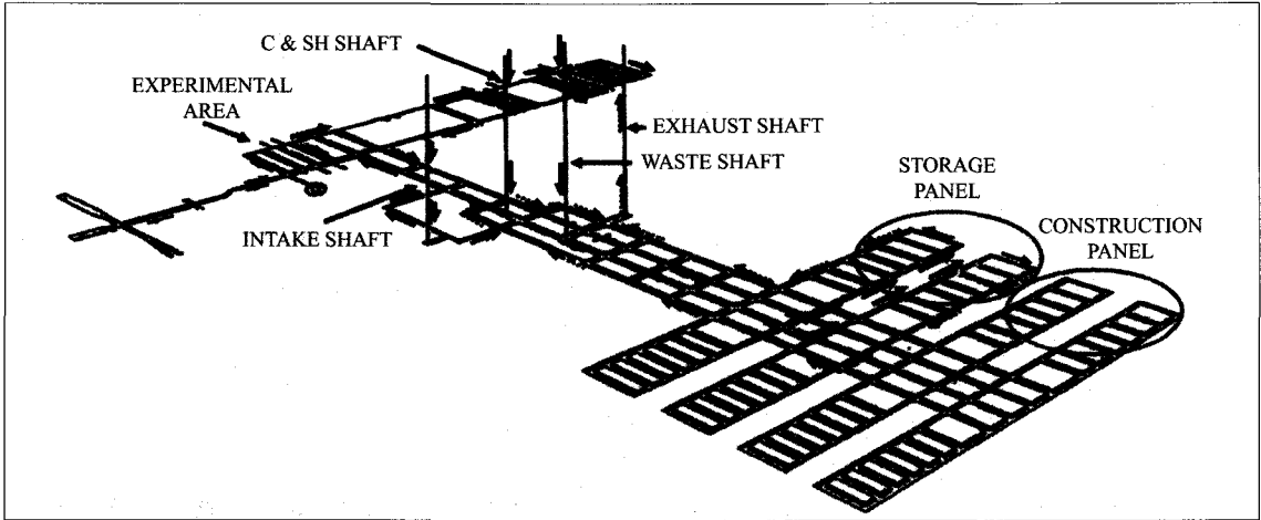
Fig. 3. Waste Isolation Pilot Plant
