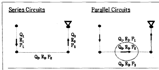
Fig. 2. Ventilation Circuits
