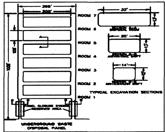
Fig. 4. Geometry of Repository Panel
