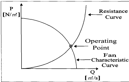
Fig. 1. Resistance Curve & Fan Characteristic Curve
