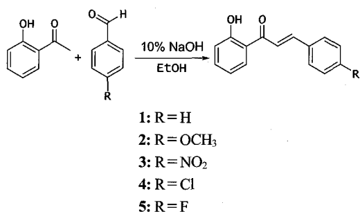
Scheme 1. Synthesis of ligands.
