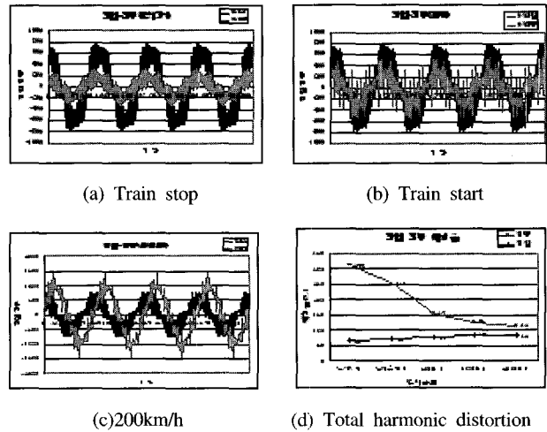
Fig. 7. Input voltage & current auxiliary power supply
