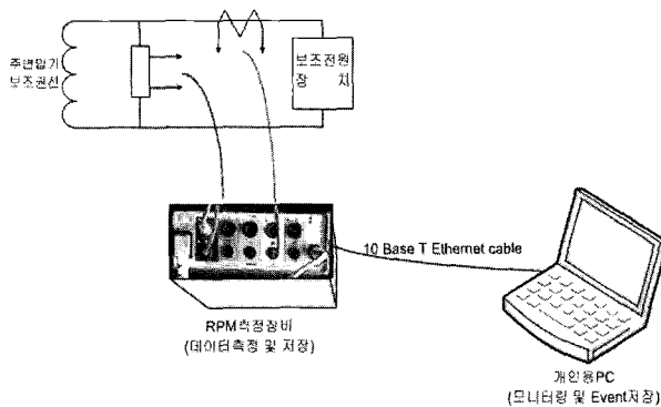
Fig. 2. Measurement of auxiliary power supply input
