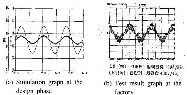
Fig. 8. Wave form of auxiliary power input for design and manufacturing
