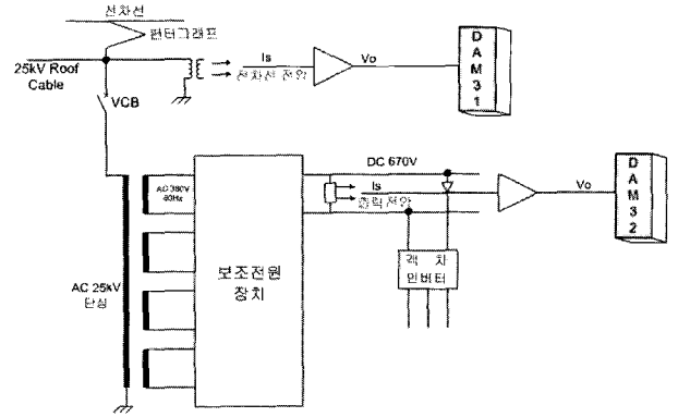
Fig. 3. Composition of measurement circuits
