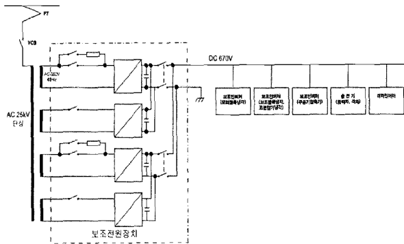
Fig. 1. Auxiliary power supply block diagram
