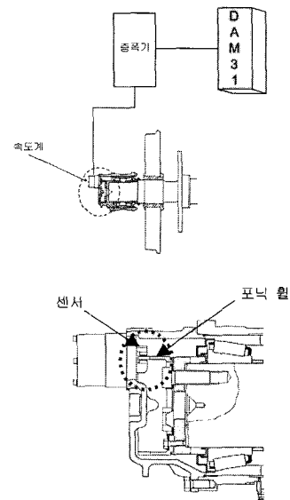
Fig. 4. Measurement of train speed
