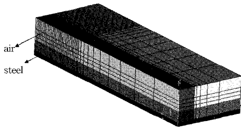
Fig. 4 Three dimensional model for electro-magnetic analysis
