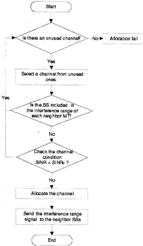
Fig. 6. Flow chart of combined algorithm.
