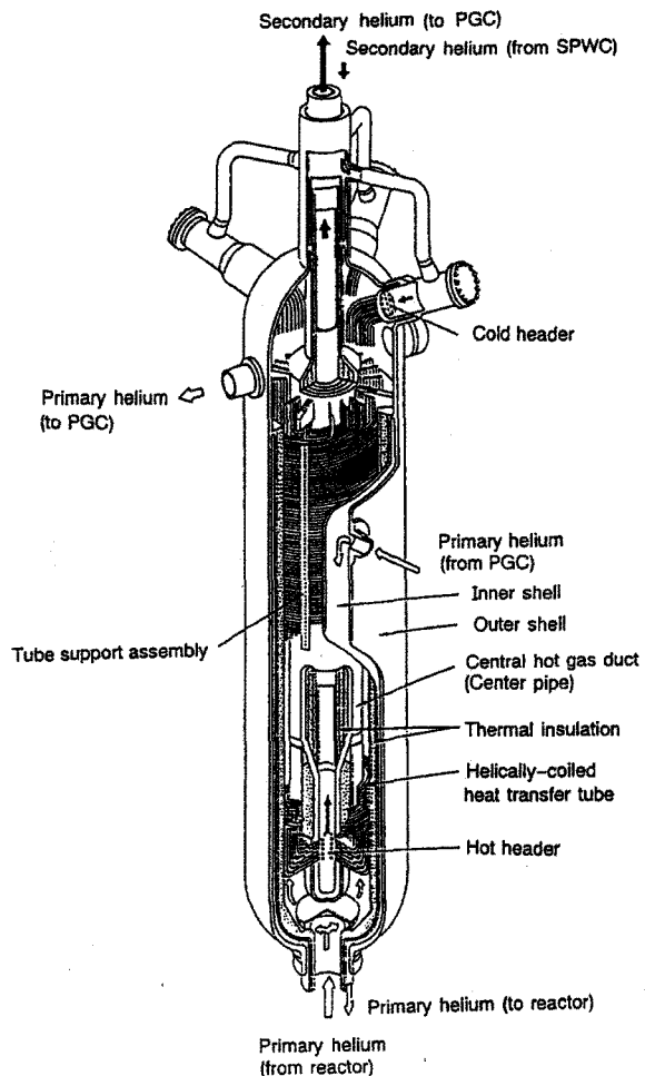
Fig. 4. Schematic View of the HTTR-IHX
