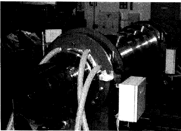
Fig. 3. Rotor of 1/3 Scale Magnetic Bearing Test
