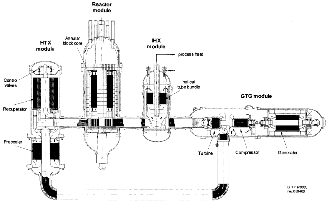
Fig. 5. System Layout of the GTHTR300C
