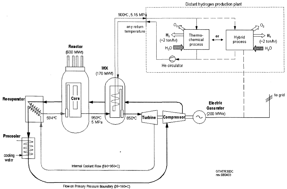
Fig. 6. Cycle Process Scheme of the GTHTR300C
