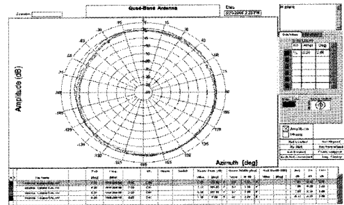
(c) H면 방사패턴(DCS) (c) Radiation pattern of H-plane (DCS)
