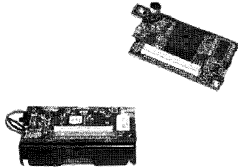
Fig. 1. Picture of sensor used in project. At the front is the MICA2 mote, at the back is the MTS300 sensor board.
