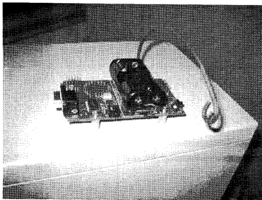
Fig. 2. Picture of MIB510 gateway which uses a serial port with base board attached.
