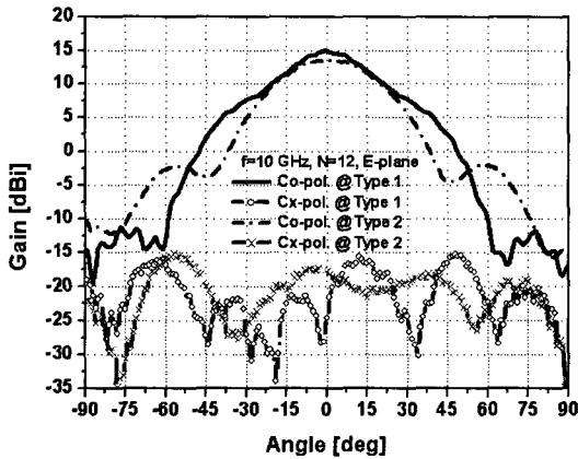
(a) E-plane
