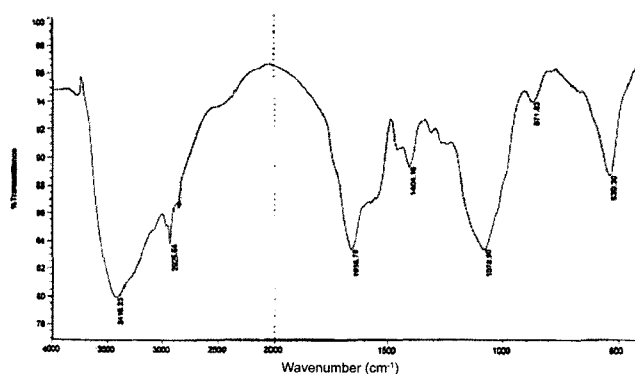
Fig. 4. FTIR spectrum of the exopolysaccharide produced by Vibrio furnissii VB0S3.
