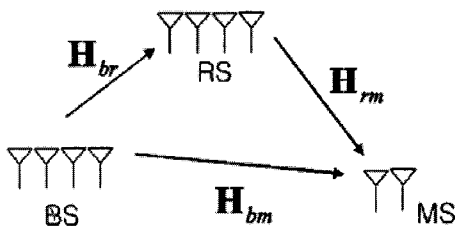
Fig. 3 Communication system mode for case 2
