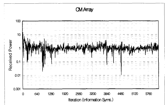
Fig. 3 The Received Power with CMA Array
