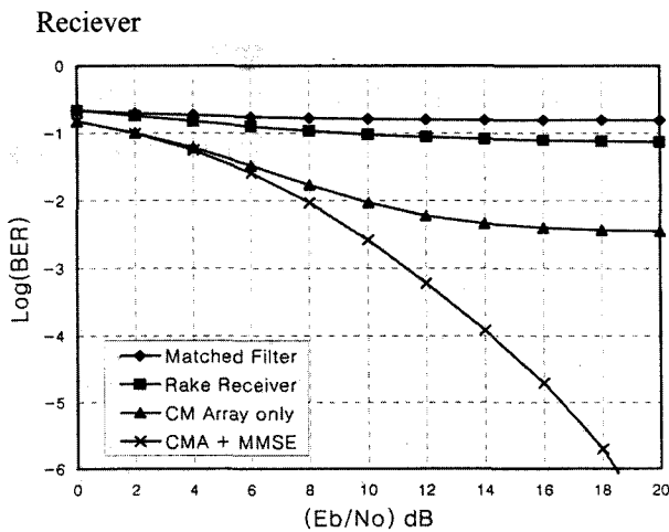
Fig. 8 BER Performance of the Several Different Receiver
