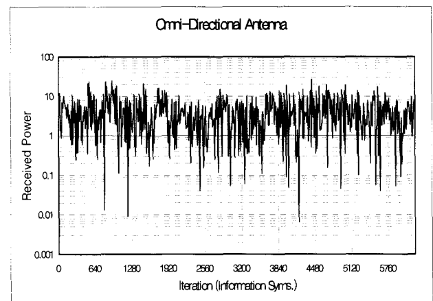
Fig. 2 The Received Power with Omni-Directional Antenna
