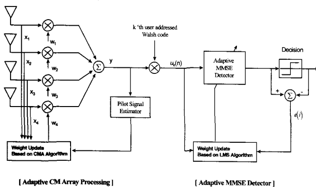
Fig. 1 The System model of CMA array cascaded by MMSE Receiver
