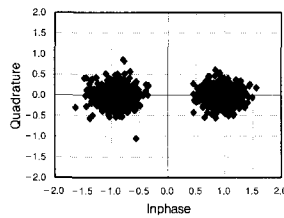
Fig. 7 CMA Array only with MMSE
