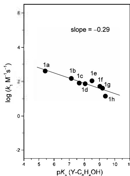
Figure 3. Plot of \log k_1 vs. \text{p}K_{\text{a}} of the conjugate acids of the leaving aryloxides for reactions of 1a-h with piperidine in 80 mol % H 2 O/20 mol % DMSO at 25.0 ± 0.1 °C. The identity of points is given in Table 2.
