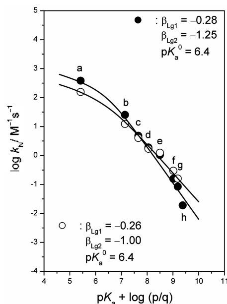
Figure 1. Bronsted-type plots for reactions of 1a-h (●) and 2a-g (○) with piperidine in 80 mol % H 2 O/20 mol % DMSO at 25.0 ± 0.1 °C. The identity of points is given in Table 1.
