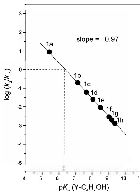
Figure 4. Plot of \log k_2 / k_{-1} vs. \text{p}K_{\text{a}} of the conjugate acids of the leaving aryloxides for reactions of 1a-h with piperidine in 80 mol % H 2 O/20 mol % DMSO at 25.0 ± 0.1 °C. The identity of points is given in Table 2.
