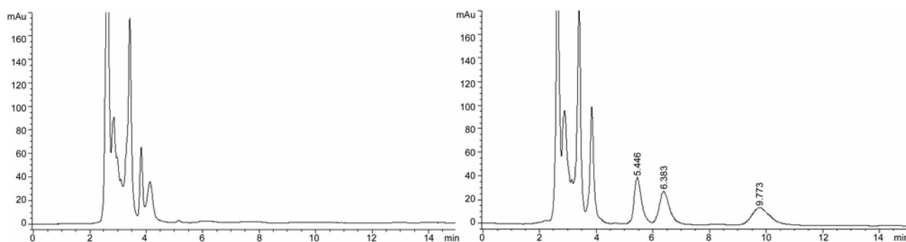
Figure 1. Chromatograms of a blank human plasma sample (the left) and a typical plasma sample spiked with IS (50 \mu g/mL, 5.446 min), L-T4 (20 \mu g/mL, 6.383 min) and D-T4 (20 \mu g/mL, 9.773 min) (the right). See experimental for chromatographic conditions.
