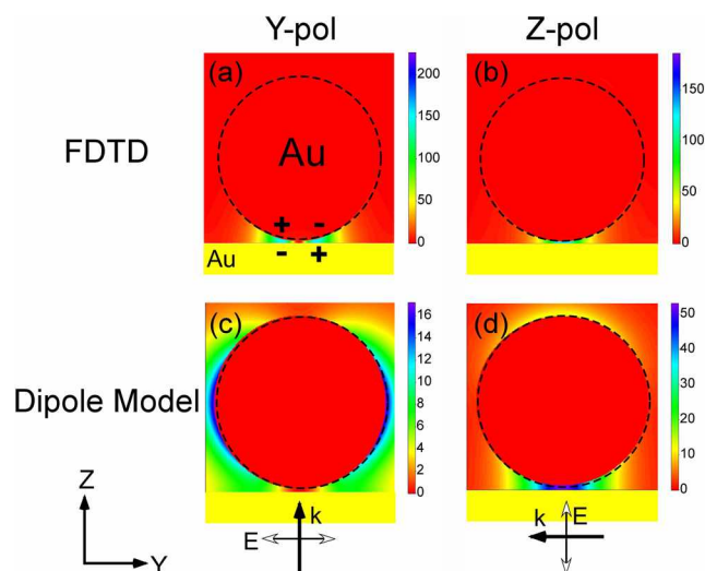
Figure 1. Local field intensity ( |E|^2 = E_y^2 + E_z^2 ) distributions around nanosphere-plane junction ( d = 5 nm) excited with y-polarized light (a and c) and z-polarized light (b and d). The (a) and (b) are the results of rigorous FDTD calculations. The (c) and (d) are the results from dipole-image dipole model calculations. Also shown are the propagation ( k ) and polarization ( E ) directions of the excitation field.
