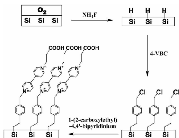
Scheme 1. The synthetic sequence of Si(111)-4-vinylbenzyl-1-(2-carboxylethyl)-4,4'-bipyridium.
