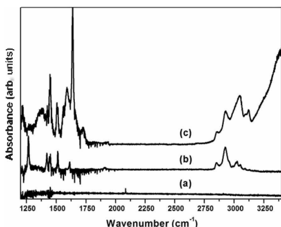
Figure 1. ATR-FTIR spectra of (a) H-Si(111), (b) 4-VBC-Si(111), and (c) Si-4-VB-VCOOH substrates.
