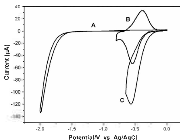
Figure 2. Cyclic voltammograms of 4-VBC-Si(111) electrode under argon atmosphere (a), and the first redox process of viologen (2+/+) at Si-4-VB-VCOOH in the absence (b) and presence (c) of molecular oxygen in 0.1 M potassium chloride electrolyte solution. Scan rate; 10 mV/S.
