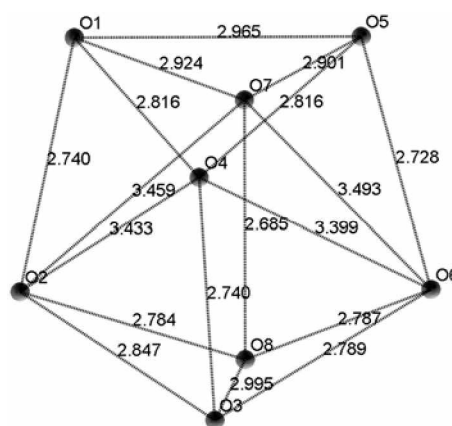
Fig. 3. The length of the polyhedron edges.
