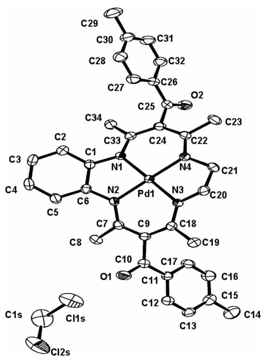
Figure 2. The molecular structure of complex 2. Selected bond lengths (Å) and angles ( ^{\circ} ) (standard uncertainties in parentheses): Pd(1)-N(1) 1.971(3), Pd(1)-N(4) 1.957(3), N(1)-C(1) 1.416(4), N(4)-C(21) 1.474(5), N(4)-C(22) 1.323(4), N(1)-C(33) 1.349(4), C(10)-O(1) 1.219(4), N(1)-Pd(1)-N(4) 95.57(1), N(2)-Pd(1)-N(1) 84.32(1), N(4)-Pd(1)-N(2) 179.08(1), N(4)-Pd(1)-N(3) 85.18(1), N(2)-Pd(1)-N(3) 94.96(1), N(3)-Pd(1)-N(1) 178.08(1).
