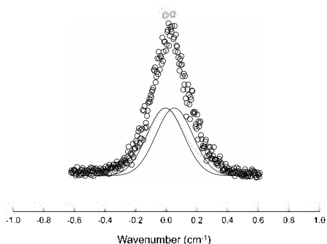
Figure 3. Doppler profile of the R_{v=0}(4) rotational transition of CN. The dotted line is the laser line profile and the solid lines are the actual Doppler profiles after deconvolution of the laser line profile.
