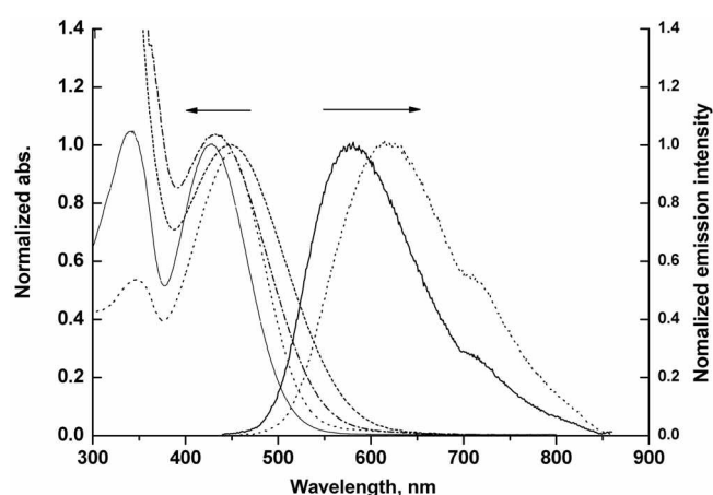
Figure 2. Absorption and emission spectra of JK-34 (solid line) and JK-36 (dot line) in ethanol and absorption spectra of JK-34 (dashed dot line) and JK-36 (short dashed line) absorbed on TiO 2 film. The emission spectra were obtained using the same solution by exciting at 429 nm for JK-34 and 450 nm for JK-36 at 298 K.
