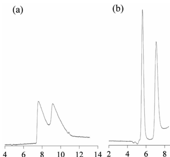
Figure 2. Enantioseparation of pindolol (7) on CDMPC using (a) acetonitrile or (b) acetonitrile + 0.1% DEA as mobile phase.
