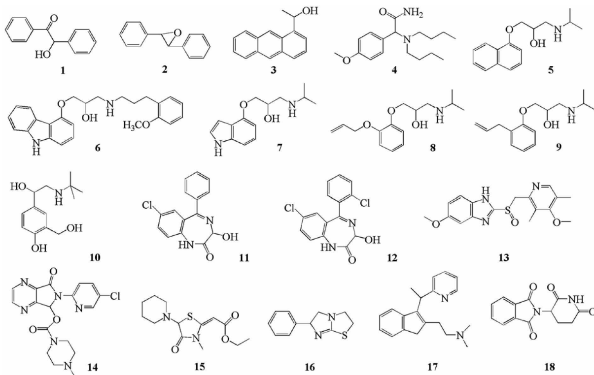
Figure 1. Structure of chiral analytes used in this study: 1. benzoin, 2. t -stilbene oxide, 3. anthryl ethanol, 4. ambucetamide, 5. propranolol, 6. carvedilol, 7. pindolol, 8. oxprenolol, 9. alprenolol, 10. salbutamol, 11. oxazepam, 12. lorazepam, 13. omeprazole, 14. zopiclone, 15. etozolin, 16. tetramisole, 17. dimetinden, 18. thalidomide.
