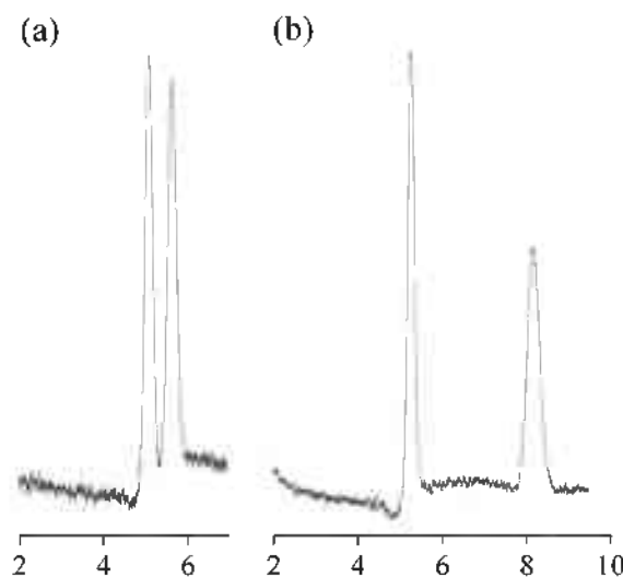
Figure 3. Enantioseparation of ambucetamide (4) on CDMPC using (a) methanol or (b) acetonitrile as mobile phase.
