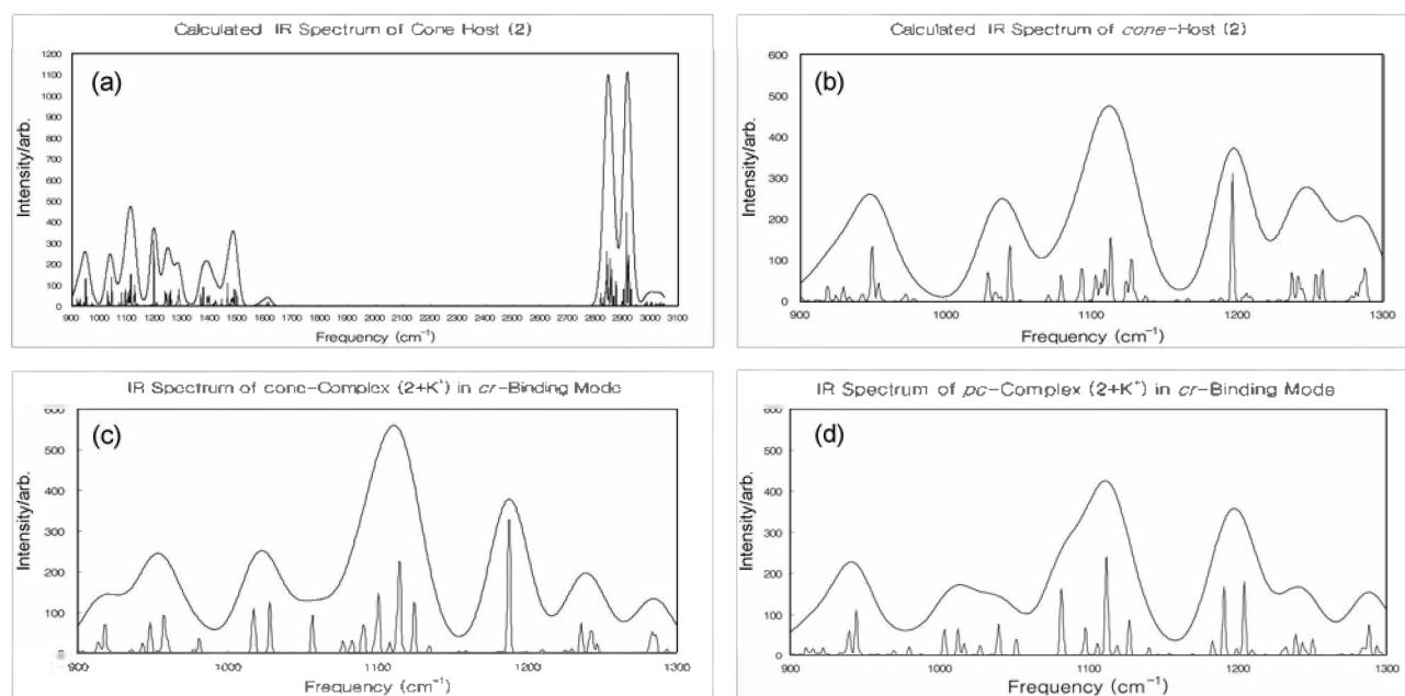
Figure 4. Calculated IR spectra of (a) the range between 900 and 3100 \text{cm}^{-1} and (b) the range between 900-1300 \text{cm}^{-1} of cone m -shaped 1,3-diethoxy- p - tert -butylcalix[4]crown-5-ether 2 as the host molecule, and (c) 2 cone +K + complex and (d) 2 pc +K + complex in cr -binding mode. In each figure, the upper trace is presented as the broadened IR spectrum assuming a Lorentzian line width of 30 \text{cm}^{-1} to simulate the experimental spectrum, and the lower spectrum as line width of 2 \text{cm}^{-1} to show the vibrational frequencies.
