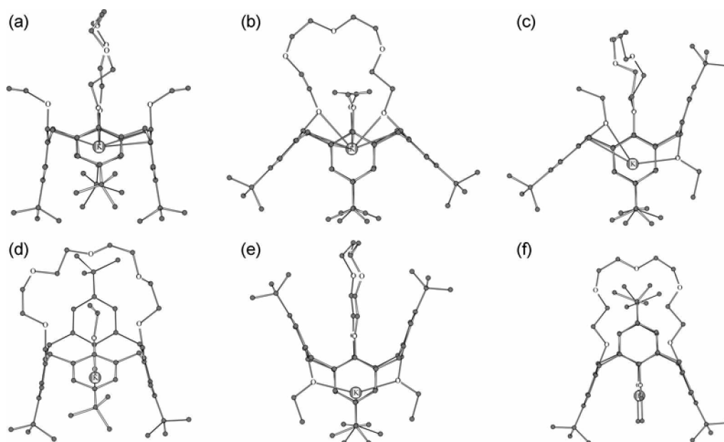
Figure 3. Ab initio calculated structures of bz -complex 2+K^+ . (a) Side view and (b) front view of cone m conformer, (c) side view and (d) front view of partial-cone conformer, (e) side view and (f) front view of 1,3-alternate conformer.
