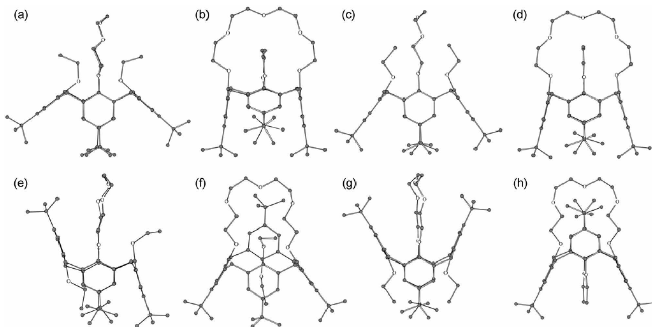
Figure 1. Ab initio calculated structures of host 1 . (a) Side view and (b) front view of cone out conformer, (c) side view and (d) front view of cone in conformer, (e) side view and (f) front view of partial-cone conformer, (g) side view and (h) front view of 1,3-alternate conformer.
