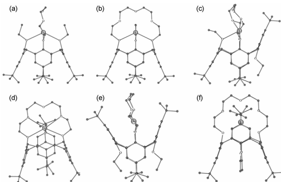
Figure 2. Ab initio calculated structures of cr -complex 2+K^+ . (a) Side view and (b) front view of cone m conformer, (c) side view and (d) front view of partial-cone conformer, (e) side view and (f) front view of 1,3-alternate conformer. Atoms that are within a certain distance (the bond proximate distance) from one another were automatically marked as bonded. 13
