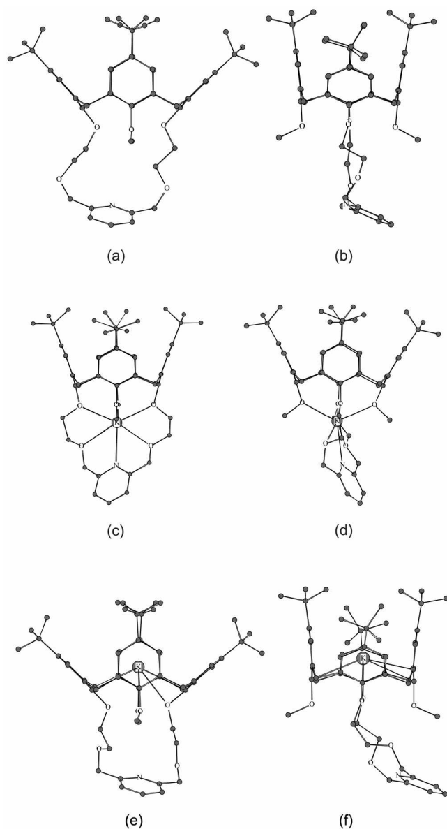
Figure 1. DFT calculated structures of cone conformer of 1 . (a) Side view and (b) front view of the cone host 1 , (c) side view and (d) front view of the cone cr -complex 1 •K + , (e) side view and (f) front view of the cone bz -complex 1 •K + . Atoms that are within a certain distance (the bond proximate distance) from one another were automatically marked as bonded. 15
