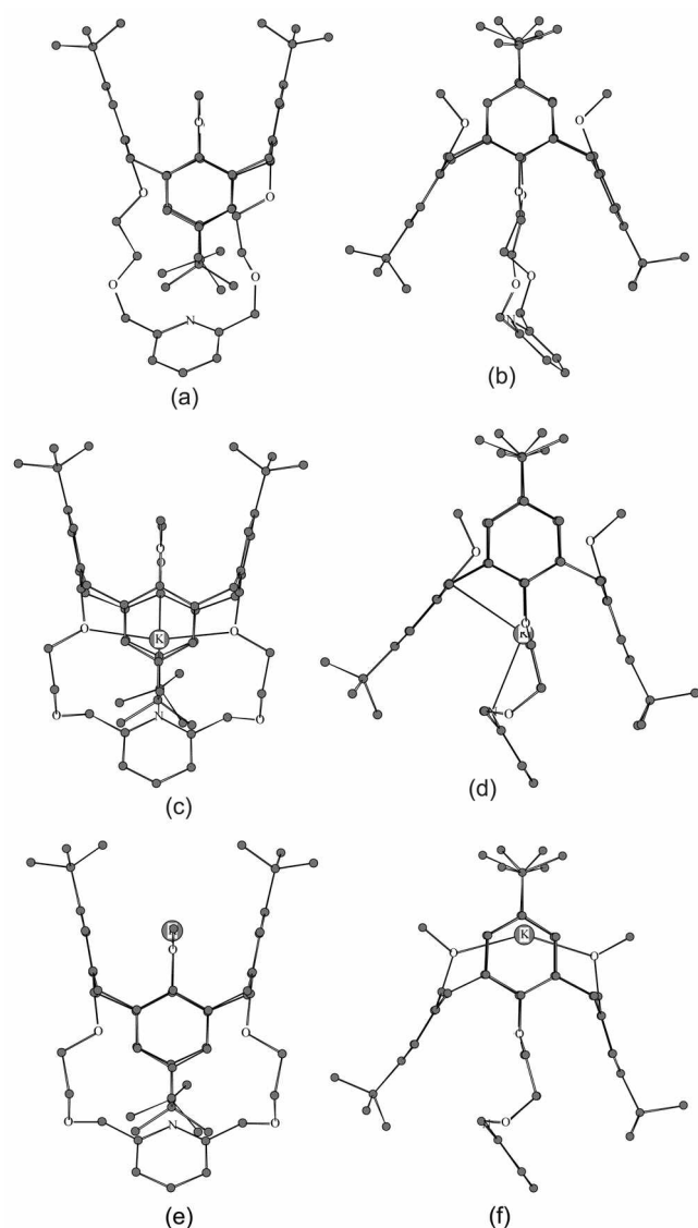
Figure 3. DFT calculated structures of 1,3-alternate conformer of 1 . (a) Side view and (b) front view of the 1,3-alternate host 1 , (c) side view and (d) front view of the 1,3-alternate cr -complex 1 •K + , (e) side view and (f) front view of the 1,3-alternate bz -complex 1 •K + .
