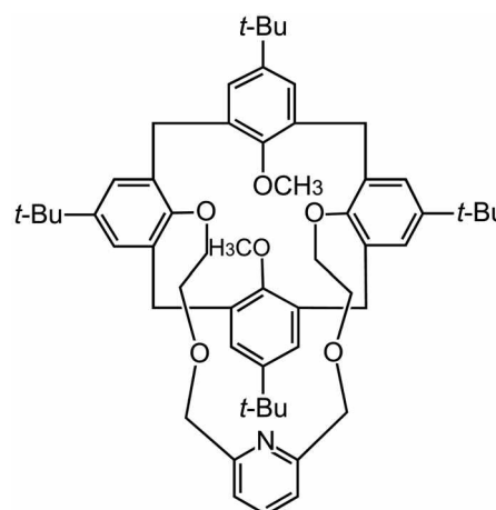
Scheme 1. Chemical drawing of p - tert -butylcalix[4]arene crown ether bridged at the lower rim with pyridyl unit ( 1 ).
