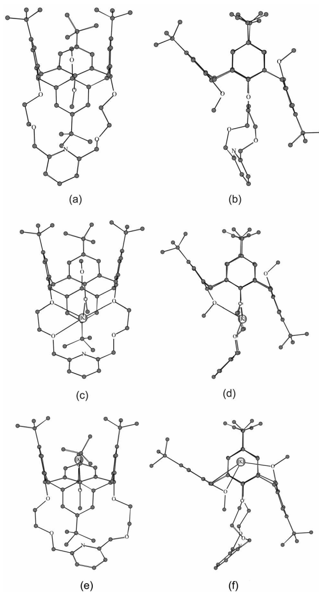
Figure 2. DFT calculated structures of partial-cone conformer of 1 . (a) Side view and (b) front view of the partial-cone host 1 , (c) side view and (d) front view of the partial-cone cr -complex 1 •K + , (e) side view and (f) front view of the partial-cone bz -complex 1 •K + .
