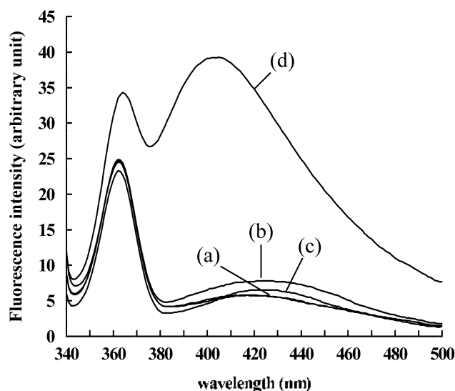
Figure 4. Fluorescence spectra of cytochrome c /H 2 O 2 system-mediated NF-L aggregation. The fluorescence spectra of the formation of dityrosine was observed when NF-L (0.25 mg/mL) was incubated with or without 10 \mu M cytochrome c and 500 \mu M H 2 O 2 . (a) NF-L control (b) NF-L + cytochrome c (c) NF-L + H 2 O 2 (d) NF-L + cytochrome c + H 2 O 2 .
