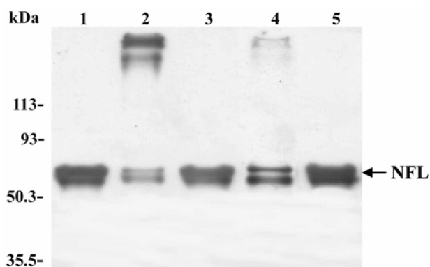
Figure 2. Effect of radical scavengers on cytochrome c /H 2 O 2 system-mediated NF-L aggregation. NF-L (0.25 mg/mL) was incubated with 10 \mu M cytochrome c and 500 \mu M H 2 O 2 in 10 mM phosphate buffer (pH 7.4) at 37 °C for 2 h in the presence of radical scavengers. Lane 1, NF-L control; lane 2, no addition; lane 3, 200 mM azide; lane 4, 200 mM formate; lane 5, 10 mM N-acetyl-L-cysteine.
