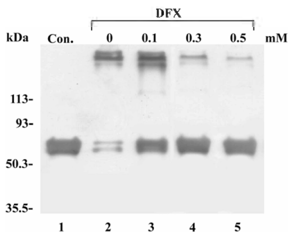
Figure 5. Effect of iron chelator on cytochrome c /H 2 O 2 system-mediated NF-L aggregation. NF-L (0.25 mg/mL) was incubated with 10 \mu M cytochrome c and 500 \mu M H 2 O 2 in 10 mM phosphate buffer (pH 7.4) at 37 °C for 2 h in the presence of iron chelator. Lane 1, NF-L control; lane 2, no addition; lane 3, 0.1 mM DFX; lane 4, 0.3 mM DFX; lane 5, 0.5 mM DFX. The positions of molecular weight markers (kDa) are indicated on the left.
