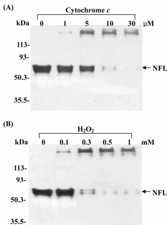
Figure 1. Aggregation of NF-L by the cytochrome c and H 2 O 2 system analyzed by immunoblotting. NF-L (0.25 mg/mL) was incubated with various concentrations of cytochrome c and various concentrations of H 2 O 2 in 10 mM phosphate buffer (pH 7.4) at 37 °C for 2 h. (A) NF-L was incubated with indicated concentrations of cytochrome c and 500 μM H 2 O 2 . (B) NF-L was incubated with 10 μM cytochrome c and indicated concentrations of H 2 O 2 . The positions of molecular weight markers (kDa) are indicated on the left.
