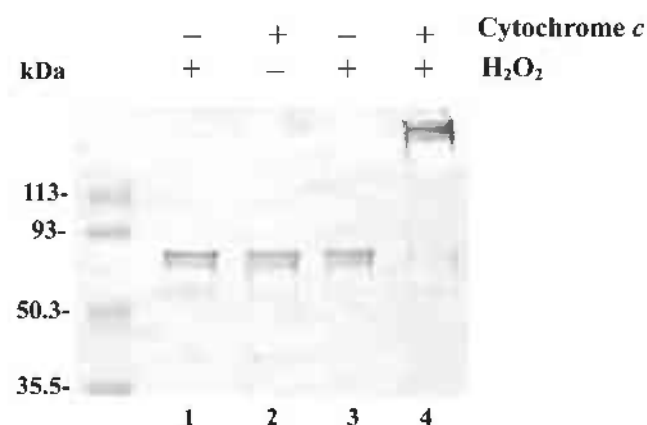
Figure 3. Immunoblotting analysis of carbonyl groups in NF-L after incubation of cytochrome c and H 2 O 2 . NF-L (0.25 mg/mL) was incubated in 10 mM phosphate buffer (pH 7.4) at 37 °C for 2 h under various conditions. After incubation, samples were derivatized DNPH as described under "Materials and methods". DNPH-derivatized proteins were subjected to SDS-PAGE for immunoblot with anti-DNP sera. Lane 1, NF-L control; lane 2, NF-L with 10 \mu M cytochrome c ; lane 3, NF-L with 500 \mu M H 2 O 2 ; lane 4, NF-L with 10 \mu M cytochrome c and 500 \mu M H 2 O 2 .
