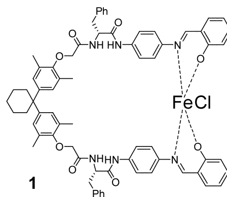
Figure 1. Structure of Metallomacrocyclic ( 1 ).
