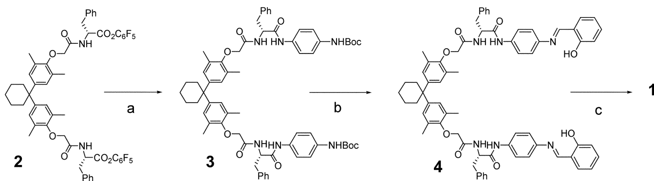
Scheme 1. Synthesis of Metallomacrocyclic ( 1 ): (a) mono-Boc-1,4-phenylene diamine, (b) TFA, then salicylic aldehyde in EtOH, (c) FeCl 3 .
