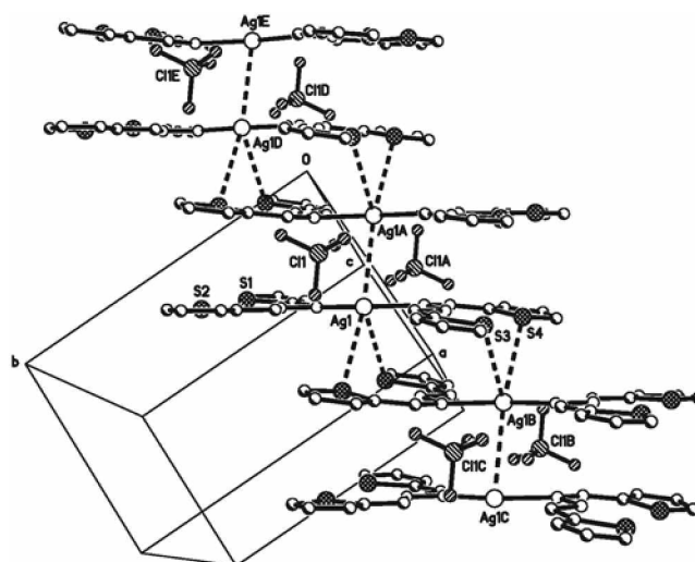
Figure 7. Packing diagram of 3 showing van der Waals interactions (dashed lines).
