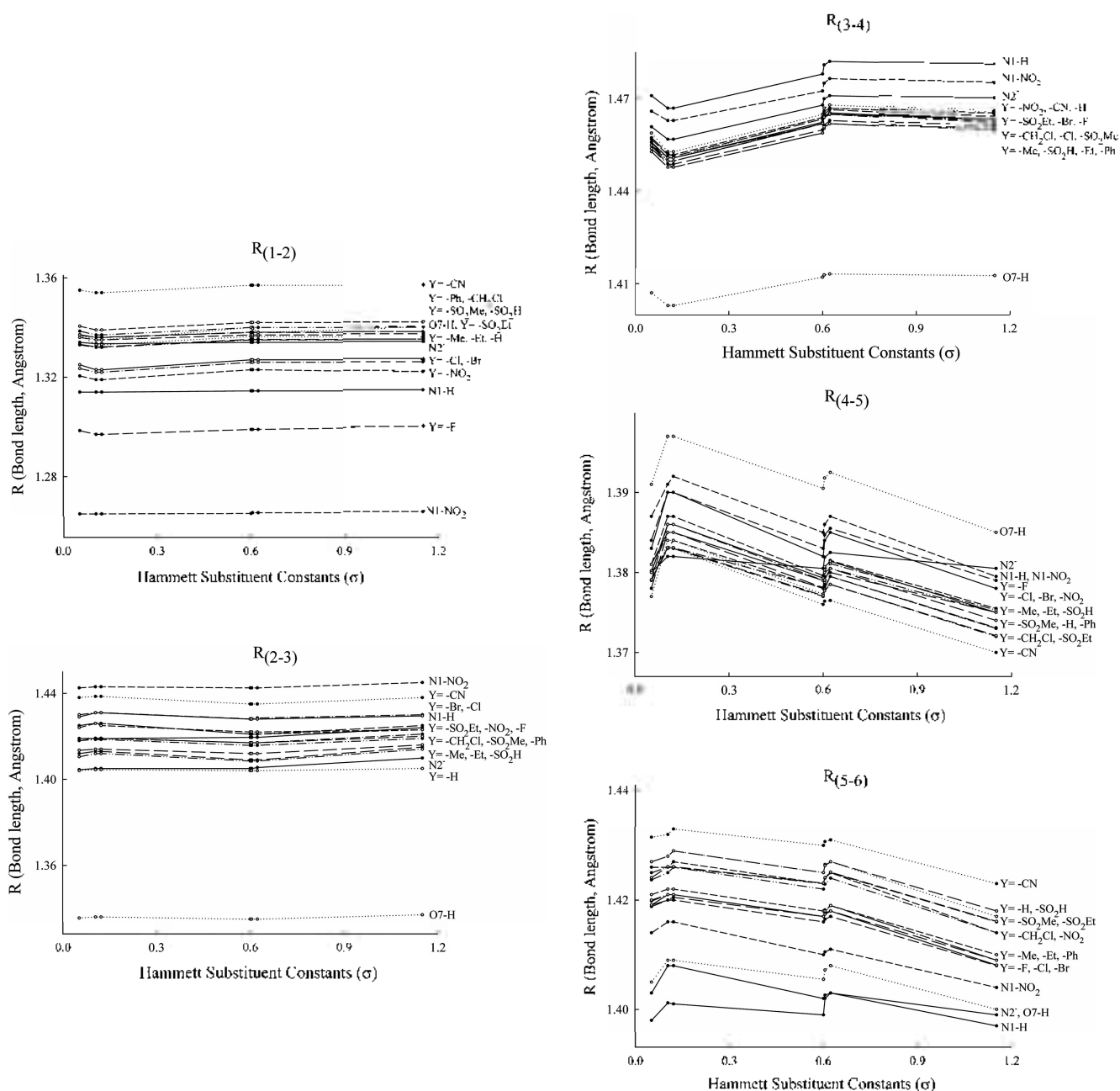
Figure 1. The variations of the bond lengths (Å) of the 4,5-disubstituted pyridazin-3-one derivatives with various functional groups at the MP2/6-31G** level. The summations of two hammett substituent constants ( \sigma_{\text{para-OPh}} + \sigma_{\text{meta-Cl}} = 0.053 ; \sigma_{\text{para-OMe}} + \sigma_{\text{meta-Cl}} = 0.105 ; \sigma_{\text{para-OEt}} + \sigma_{\text{meta-Cl}} = 0.123 ; \sigma_{\text{para-Cl}} + \sigma_{\text{meta-Cl}} = 0.60 ; \sigma_{\text{para-Br}} + \sigma_{\text{meta-Cl}} = 0.605 ; \sigma_{\text{para-Br}} + \sigma_{\text{meta-Br}} = 0.623 ; \sigma_{\text{para-NO}_2} + \sigma_{\text{meta-Cl}} = 1.151 ) of para - and meta -substituents are scaled on the X-axis. N2, N1, and O7: the position of the atoms on the six-membered ring.
