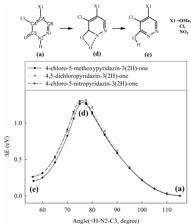
Figure 3. The energy barrier (eV) for the proton transfer ( \angle\text{H-N2-C3} = 56\text{--}115 degree) from (N2-H) at the 2-position to C=O on the 4,5-disubstituted pyridazin-3-one derivatives at the MP2/6-311+G** level.
