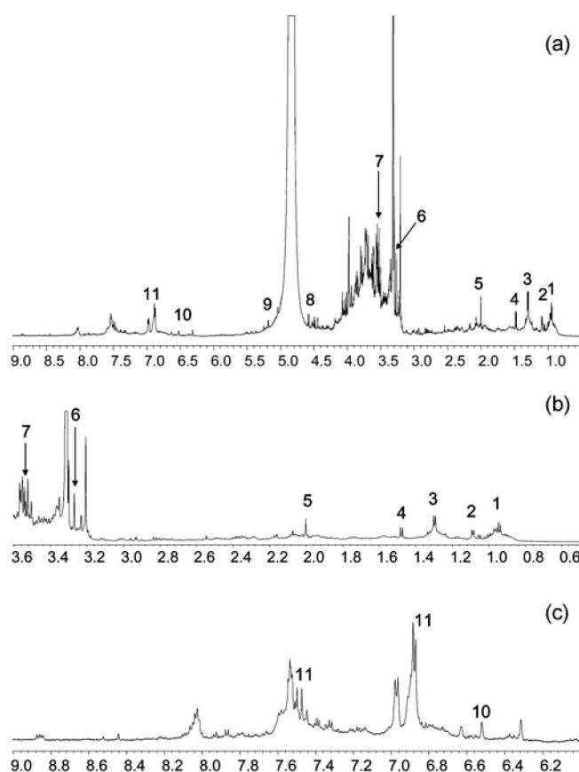
Figure 1. Representative 1 H NMR spectra of the total (a), aliphatic (b), and aromatic (c) regions of the 50% methanol fraction of a safflower sample. IS: internal standard, w: residual water, 1: fatty acid (terminal CH 3 ), 2: valine, 3: lactic acid, 4: alanine, 5: acetic acid, 6: choline derivative, 7: glycine, 8: \beta -glucose, 9: \alpha -glucose, 10: fumaric acid, 11: safflower yellow derivatives.
