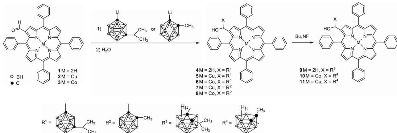
Scheme 1. Synthesis of neutral and anionic carboranylporphyrins.
