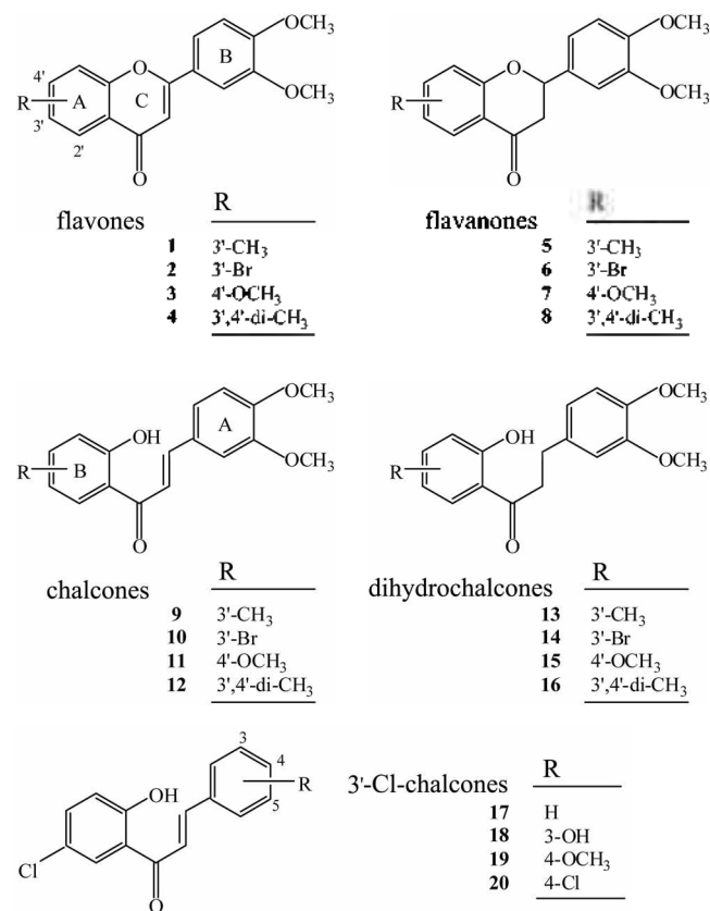
Figure 1. Chemical Structures of Tested Compounds.
