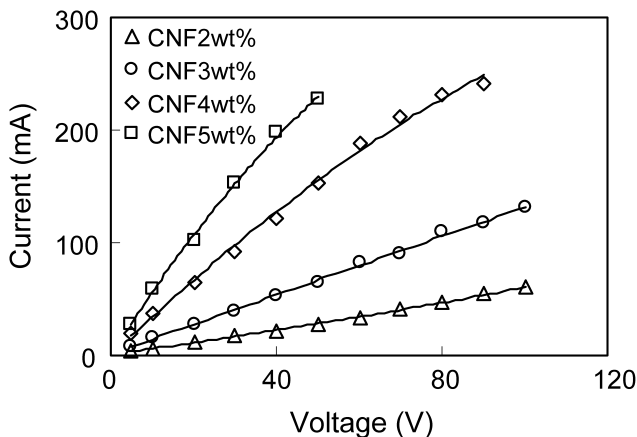
Figure 3. Relations between current and voltage for CNF/UPR nanocomposites.
