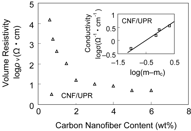
Figure 2. Relationship between electrical volume resistivity and CNF content for the CNF/UPR nanocomposites.
