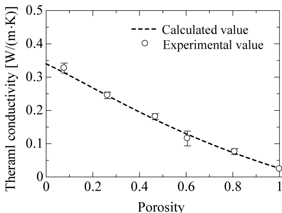
Figure 4. Measured thermal conductivity of BFGC and calculated values from equation (1).
