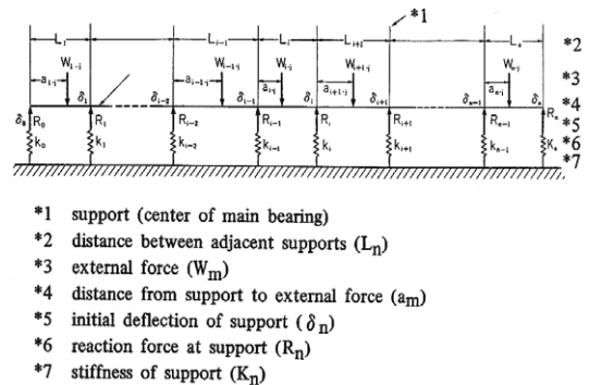
Fig. 12 Continuous beam
