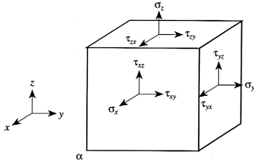
Fig. 1 Stresses in cartesian coordinate system
