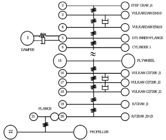
Fig. 8 Mass spring system for torsional vibration
