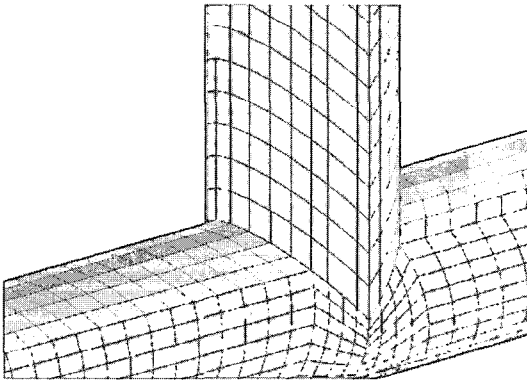
Fig. 8 Mesh configuration
