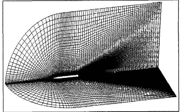
Fig. 2 Multi-block grid
