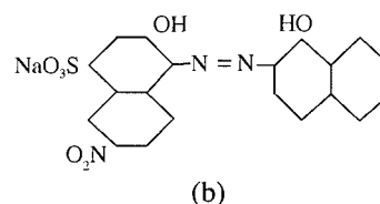
Figure 1. (a) Chemical structure of Neolan Red GRE 200 % (C.I. Acid Red 183), (b) chemical structure of Eriochrome Black T 250 % (C.I. Mordant Black 11).
