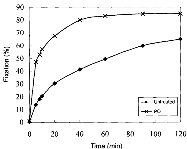
Figure 9. Fixation curve of different wool samples with reactive dye.
