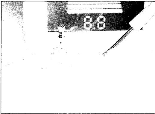
Figure 1. Alginate model.
