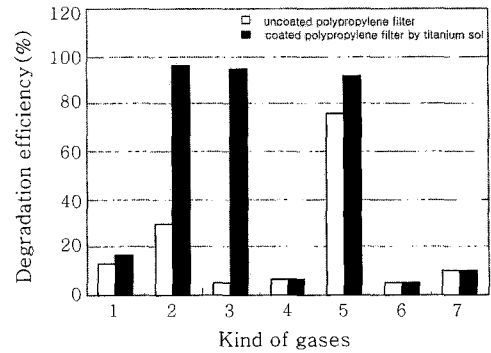
Figure 7. Degradation efficiency of formaldehyde (1), ammonia (2), trimethylamine (3), methylmercaptan (4), acetic acid (5), benzene (6), and toluene (7).
