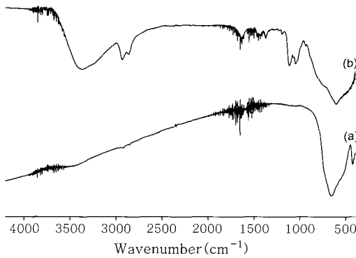
Figure 3. FTIR spectra of TiO 2 (a) and titanium complex (b).
