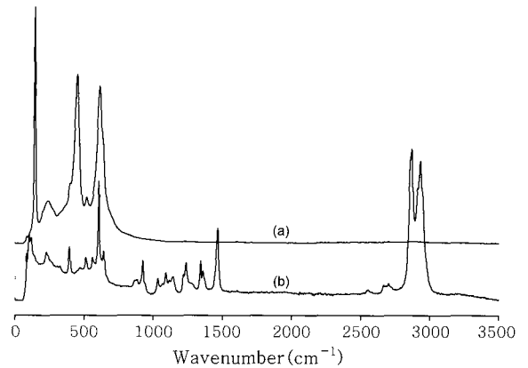
Figure 4. Raman spectra of TiO 2 (a) and titanium complex (b).
