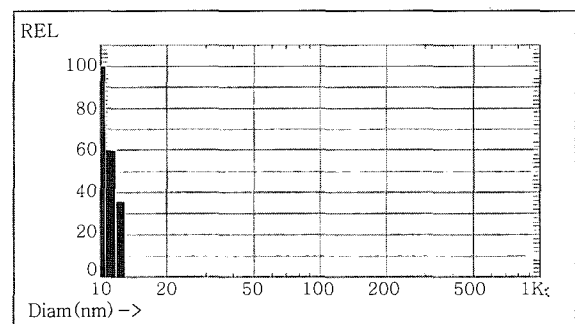
Figure 1. Particle size distribution of titania sol.
