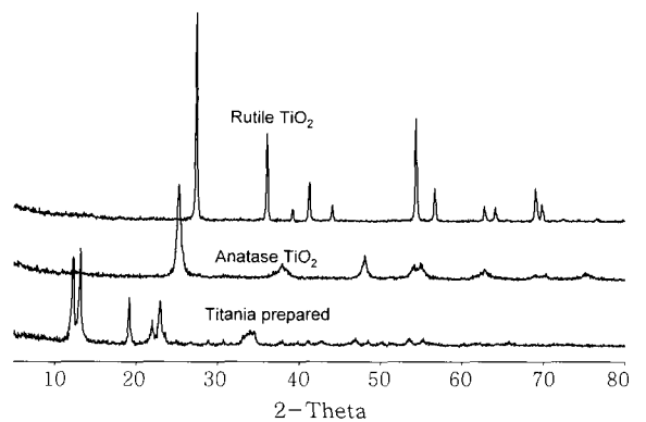
Figure 5. XRD diffraction pattern of titania prepared in this study.
